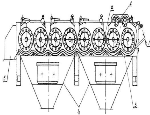
Figure 1. Cross-sectional diagram of the imperfect 1XK fine-grained cleaning equipment. 1 supply roller, 2 pile drum, 3 mesh surface, 4 dirt bunker, 5 tray
