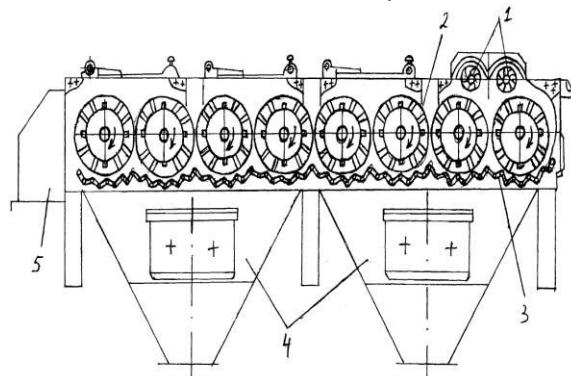
Figure 2. Cross-sectional diagram of the improved 1XK fine-grained cleaning equipment. 1 supply roller, 2 pile drum, 3 mesh surface, 4 dirt hopper, 5 tray
